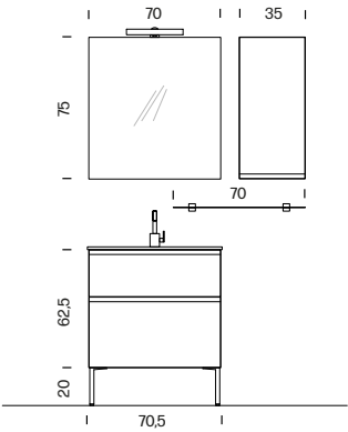
Scocca e frontali: 208 Gesso nobilitato Lavabo consolle "Ibiza" in Minera-Kolor (K4 Zante-ge) L 70,5 cm Specchiera "Wap", finitura "brill" Faretto "Roll 30" a led 4000K L 70,5+35 x P 51,5/20,8 cm Structure and doors: 208 Gesso melamine "Ibiza" console in Minera-Kolor (K4 Zante-ge) W 70.5 cm "Wap" mirror in "brill" finish "Roll 30" spotlight with led 4000K W 70.5+35 x D 51.5/20.8 cm
